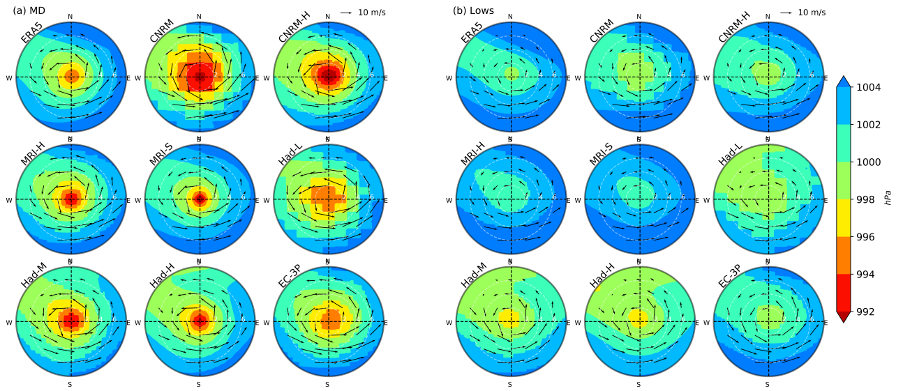
Supplementary Figure 1. Vortex-centered composites of mean sea level pressure (MSLP, shading) and horizontal wind at 850 hPa (vectors) for (a) monsoon depressions (MD) and (b) monsoon lows for observations (ERA5) and each of the individual HighResMIP models.
