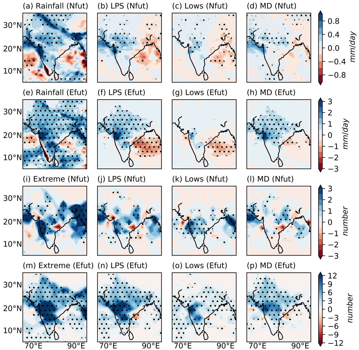
Supplementary Figure 7. Projected changes between the historical (1980-2009) and near-future (2020-2049) periods in (a) total summer (June-September) precipitation, (b) summer precipitation associated with LPS, (c) summer precipitation associated with monsoon lows, and (d) summer precipitation associated with monsoon depressions. Panels (e-h) are the same as (a-d) but for changes between the historical and extended-future (2070-2099) periods. Panels (i-p) are the same as (a-h) but for the number of extreme precipitation events during summer, with these events defined as days with precipitation greater than 150 mm. Stippling shows regions where at least 75% of the models have the same sign of change. The precipitation associated with LPS is the precipitation falling within 8^\circ of the centers of all LPS, accumulated along the tracks of those LPS; extreme events associated with LPS are the total number of extreme events that occur within 8^\circ of the storm center.
