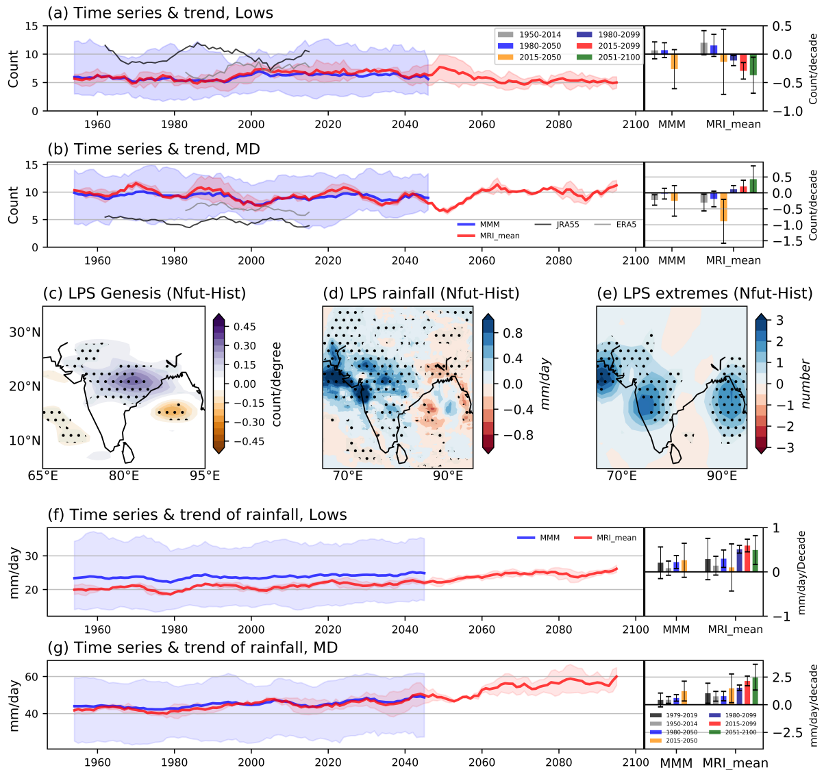
Supplementary Figure 4. Results of various analyses repeated without the HadGEM3 models, due to their strong negative bias in the number of LPS. Time series (left) and trends (right) of the number of (a) monsoon lows and (b) monsoon depressions for the multi-model means of the models having, respectively, extended-future projections to 2100 (the MRI-H and MRI-S models, thick red) and near-future projections to 2050 (blue line). Shading shows the spread across the models, and the thin black and gray lines show the JRA55 and ERA5 reanalyses. Multi-model mean changes in the (c) genesis density of all LPS, (d) summer precipitation associated with LPS, and (e) number of extreme precipitation events associated with LPS from the historical period (1980-2009) to the near future period (2020-2049). Stippling shows where at least 75% of the models have the same sign of change. Time series (left) and linear trends (right) of precipitation averaged within 3^\circ of the vortex center for (f) monsoon lows and (g) monsoon depressions in the multi-model means of the models having, respectively, extended-future projections to 2100 (the MRI-H and MRI-S models, red lines) and near-future projections to 2050 (blue lines). Shading shows the spread across the models, time series are nine-year running means, and error bars represent a 90% confidence interval. All multi-model means in this figure were calculated excluding the HadGEM3 models.
