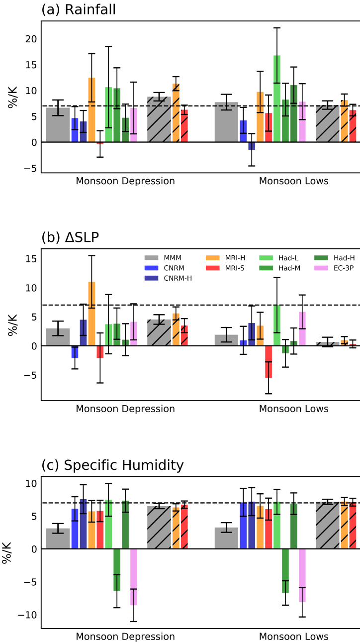
Supplementary Figure 6. Relative changes, normalized by the regional-mean surface air warming over the South Asian region (in %/K), in (a) precipitation averaged over the central region of LPS, (b) the radial difference in mean sea level pressure between the LPS center and its surroundings, and (c) specific humidity at 850 hPa averaged over the central region of LPS. Bars with diagonal hatching represent changes between the historical (1980-2009) and extended-future periods (2070-2099), while bars without hatching represent changes between the historical and near future (2020-2049) periods. The horizontal dashed line marks the 7%/K rate of change. In (a) and (c), quantities were averaged horizontally within 3^\circ of the vortex center.
