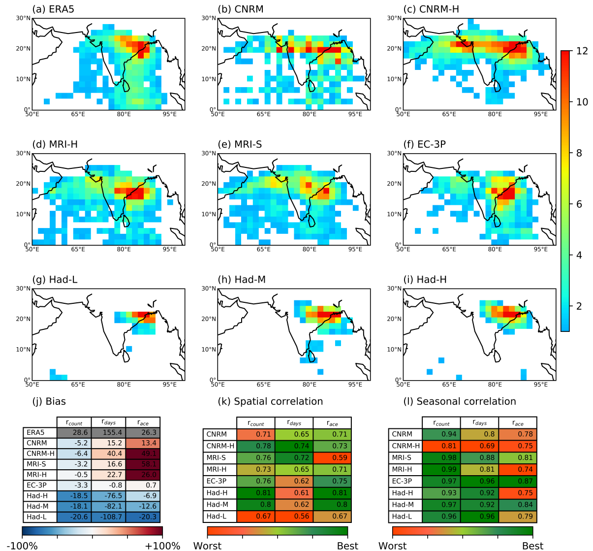
Supplementary Figure 3. Track density of low pressure systems in all seasons in (a) the ERA5 reanalysis and (b-i) individual HighResMIP models. Units are 6-hourly storms fixes per 2^\circ \times 2^\circ gridbox per year. (j) Bias in annually averaged low pressure system metrics (storm count, number of days on which storms exist, and accumulated cyclone energy [ACE]) for the models; grey-colored boxes (first row) show total values in ERA5, and subsequent rows show bias relative to ERA5, with numbers indicating absolute bias and colors the relative bias (normalized by the ERA5 value). (k) Spatial and (l) temporal correlation coefficients between the models and ERA5 of the monthly climatology of the same metrics used in (j); green and red colors range from the highest to the lowest correlation coefficients achieved across the model ensemble. The plots and matrices are generated using the standard functionalities and metrics provided by the CyMeP packages[1]
