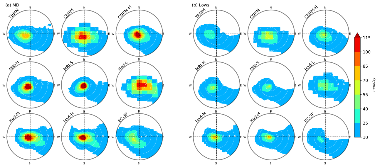
Supplementary Figure 2. Vortex-centered composites of precipitation (shading) for (a) monsoon depressions (MD) and (b) monsoon lows for observations (TRMM) and each of the individual HighResMIP models.
