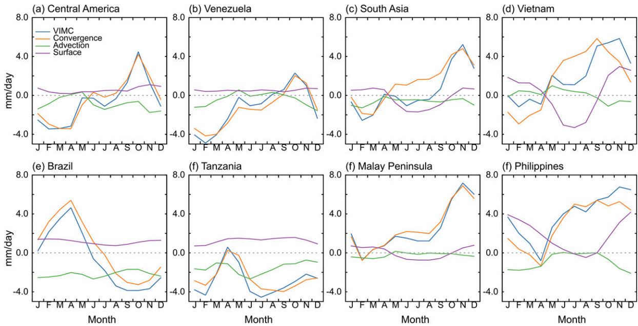
FIG. 10. The climatological annual cycle of the advection, convergence, and surface terms calculated in the budget of moisture convergence using ERA5 monthly means for each of the autumn monsoon regions.
