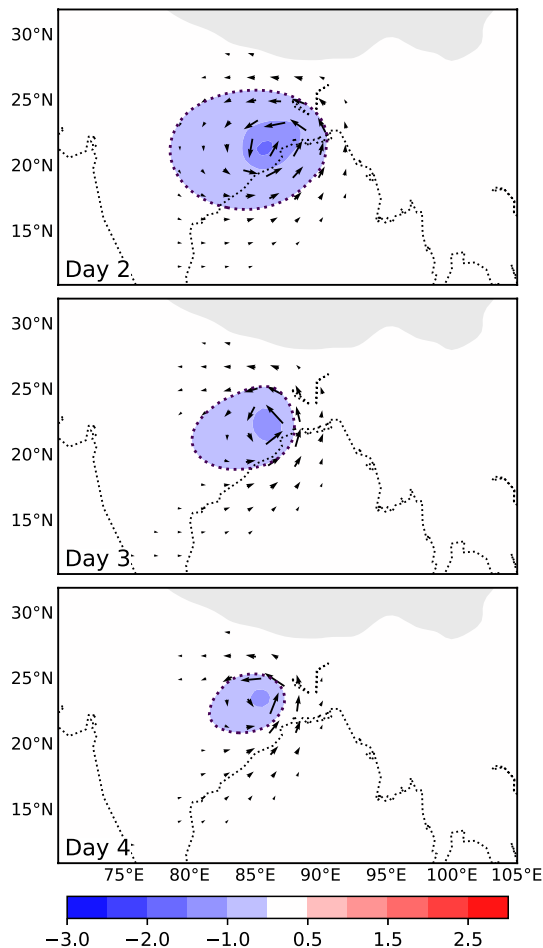
FIGURE 13 As Figure 12, but with the resting basic state [Colour figure can be viewed at wileyonlinelibrary.com]
