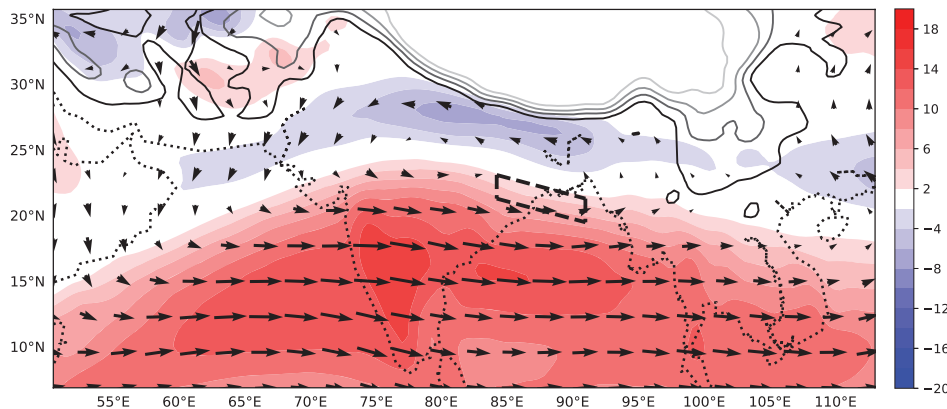
FIGURE 1 Basic state zonal wind at 3.1 km ( \bar{U} , m/s, shading), basic state wind at 3.1 km ( \bar{V} , vectors), and height of topography (contours every 1.0 km). The dashed box shows the region where heating is applied in Experiment C
