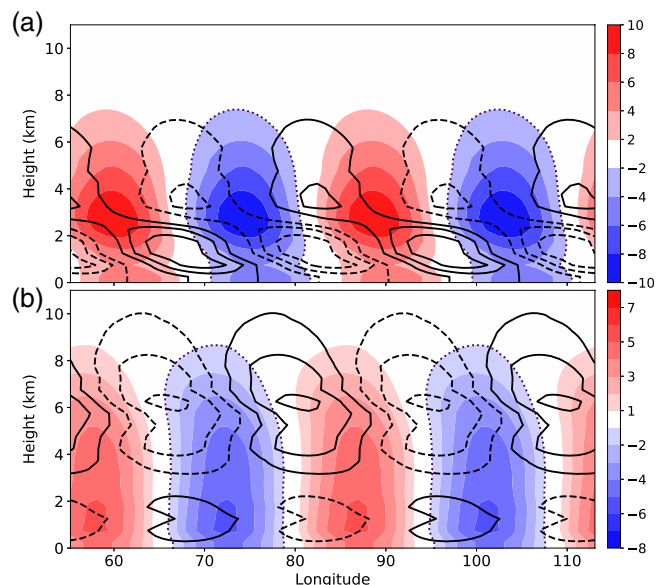
FIGURE 4 Longitude–height cross-section for Experiment A showing perturbation wind ( v' , shading, m/s) and perturbation potential temperature ( \theta' , contours) for the 3,200 km wavelength normal mode at (a) 25.7°N and (b) 21.2°N. The \theta' contour interval is (a) 1.6 K and (b) 0.63 K, with the zero contour excluded. Negative values of v' are enclosed with a dotted line. Note the change in the shading scale for the wind [Colour figure can be viewed at wileyonlinelibrary.com ]
