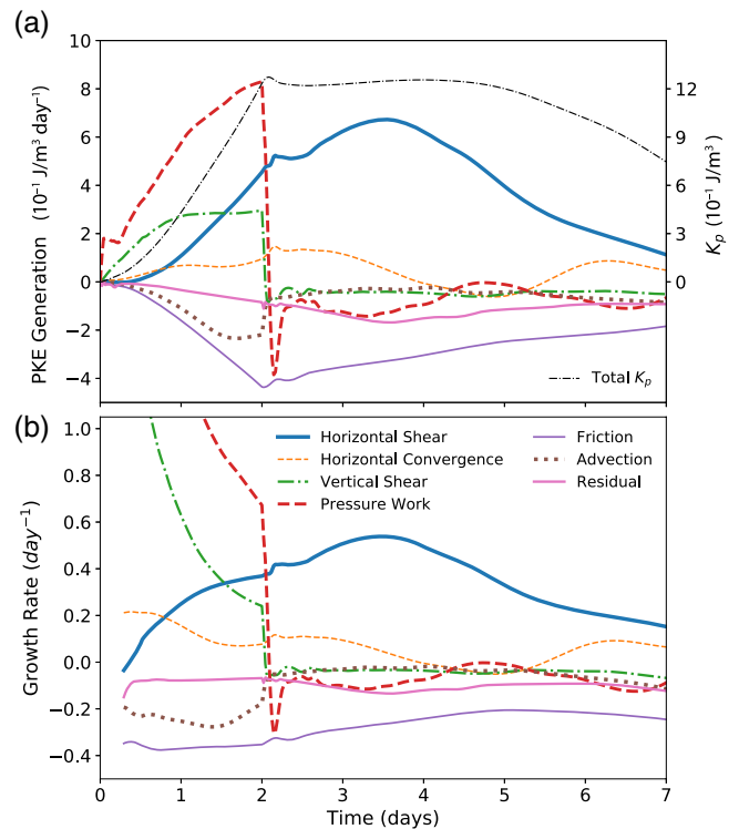
FIGURE 16 Experiment C. Terms in K_p budget (Equation 16) using the monsoon basic state: (a) shows K_p generation rates and total K_p and (b) growth rates. [Colour figure can be viewed at wileyonlinelibrary.com ]
