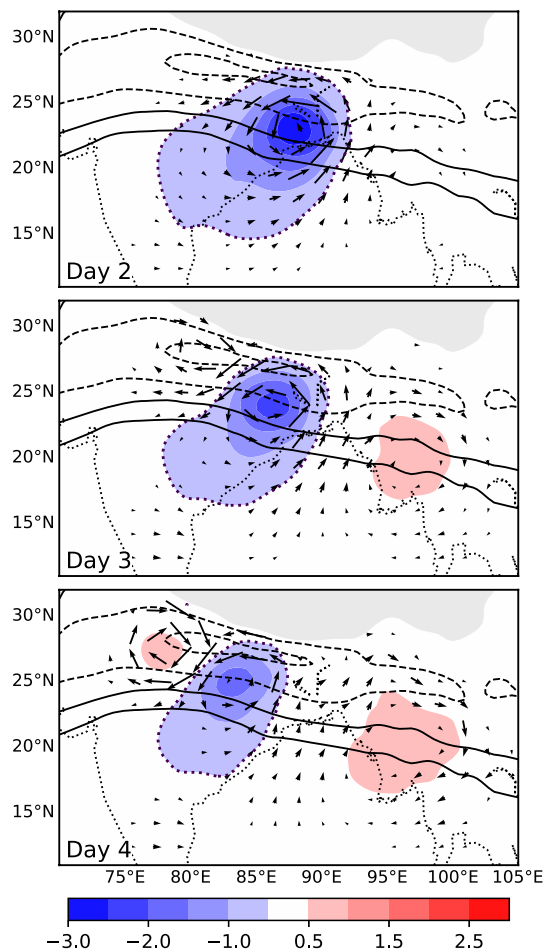
FIGURE 12 Experiment C. Perturbation pressure ( p' , shading, hPa), perturbation winds ( \mathbf{v}' , vectors), and basic state zonal wind ( \bar{U} , contours every 4 m/s between -6 m/s and +6 m/s), all at 3.1 km, at 2, 3, and 4 days into the simulation with a basic state representative of the monsoon region. Negative values of p' are enclosed with a dotted line and regions below the terrain height are masked in grey [Colour figure can be viewed at wileyonlinelibrary.com ]
