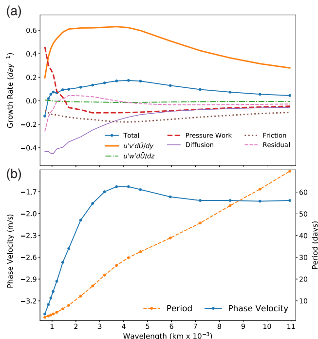
FIGURE 5 Experiment A. As a function of wavelength, (a) growth rates ( \text{day}^{-1} ) for individual terms in Equation 16 and (b) zonal phase velocity and period. The individual experiments used to construct this relationship are marked by dots in the total growth rate for (a) and in both curves for (b) [Colour figure can be viewed at wileyonlinelibrary.com ]
