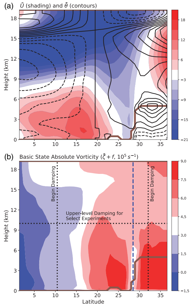
FIGURE 2 Latitude–height cross-section at 87°E of the (a) basic state zonal winds ( \bar{U} , shading, m/s) and basic state potential temperature ( \bar{\theta} , contours every 1.3 K with solid lines indicating positive values) and (b) basic state absolute vorticity ( \bar{\zeta} + f , shading, \text{s}^{-1} ). The topography is outlined in brown in both plots. The dotted black lines in (b) show the location of the boundary conditions used for some of the experiments in Experiment A. The dashed blue line shows the location north of which the basic state fields are set to a constant in Experiment A. Section 3.1 gives further details
