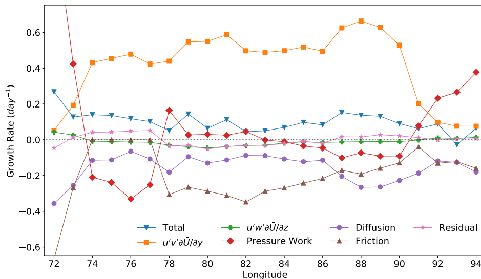
FIGURE 6 Experiment A. Growth rates as a function of longitude for individual terms in Equation 16. The individual experiments used to construct this relationship are marked by the various symbols. For presentation, the values for pressure work ( 1.24 \text{ day}^{-1} ) and friction ( -0.67 \text{ day}^{-1} ) at 72^\circ\text{E} are outside the panel [Colour figure can be viewed at wileyonlinelibrary.com ]
