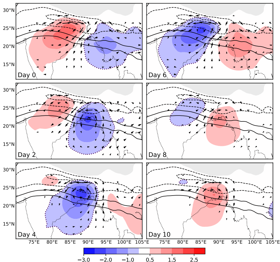
FIGURE 7 Experiment B. Time evolution from day 0 to day 10 of perturbation pressure ( p' , shading, hPa), perturbation winds ( \mathbf{v}' , vectors), and basic state zonal wind ( \bar{U} , contours every 4 m/s between -6 m/s and +6 m/s), all at 3.25 km. Negative values of p' are enclosed with a dotted line and regions below the terrain height are masked in grey [Colour figure can be viewed at wileyonlinelibrary.com ]
