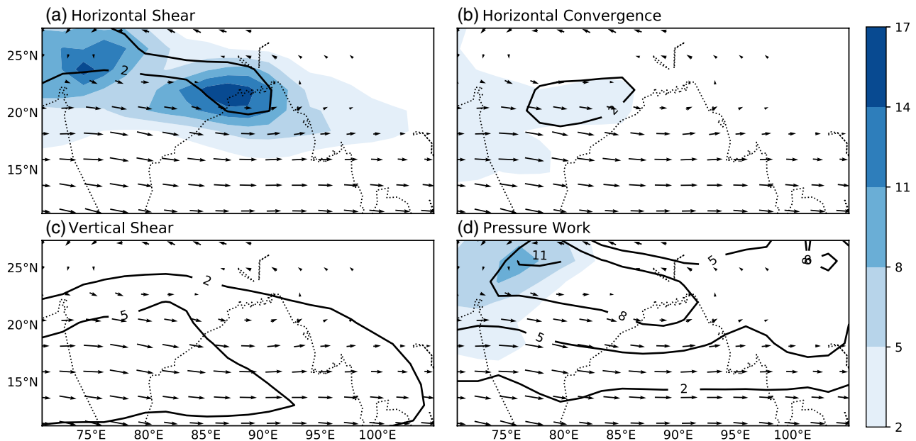
FIGURE 17 Experiment C. Basic state winds at 3.1 km (vectors) and total perturbation kinetic energy ( \text{J/m}^3 ) generated by selected terms in Equation 16. Contours show values integrated from 0 to 48 hr of each simulation and shading shows values integrated from 51 to 144 hr. Section 5.3 gives more details [Colour figure can be viewed at wileyonlinelibrary.com ]
