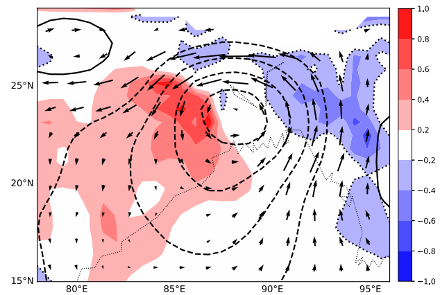
FIGURE 9 Experiment B. Perturbation vertical velocity averaged from 1.0 to 5.0 km ( w' , shading, cm/s) and perturbation winds at 3.25 km ( v' , vectors) at day 4. Negative values of w' are enclosed with a dotted line [Colour figure can be viewed at wileyonlinelibrary.com ]
