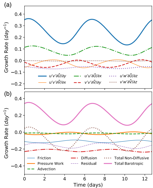
FIGURE 11 Experiment B. Growth rate ( \text{day}^{-1} ) as a function of time with dates corresponding to Figure 7. (a) shows the barotropic terms from Equation 16 and (b) shows the remaining terms in Equation 16, along with the sum of the barotropic terms [Colour figure can be viewed at wileyonlinelibrary.com ]
