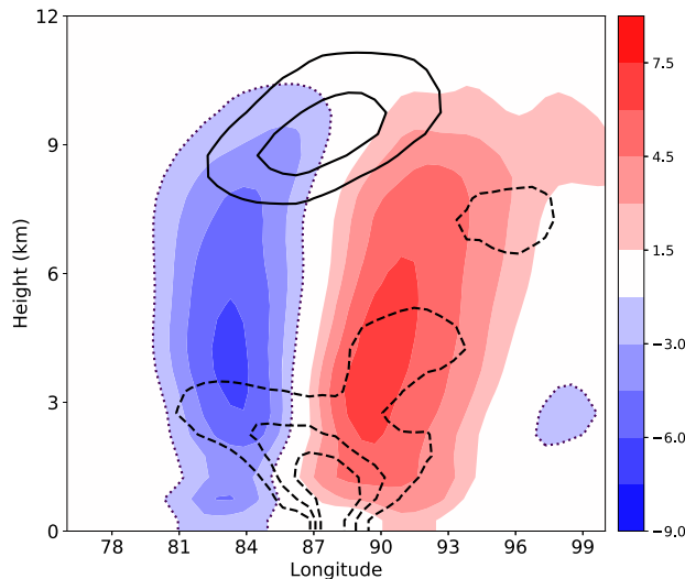
FIGURE 8 Experiment B. Longitude–height cross-section of the component of perturbation wind orthogonal to the cross-section (shading, m/s) and perturbation potential temperature ( \theta' , contours every 1 K excluding zero) at day 5. Negative values of v' are enclosed with a dotted line. This cross-section is rotated 30° clockwise from a line of constant latitude and the fields are averaged for 225 km on either side of the cross-section. Because of this rotation, longitude on the x -axis corresponds to 0.87 of its normal length [Colour figure can be viewed at wileyonlinelibrary.com ]
