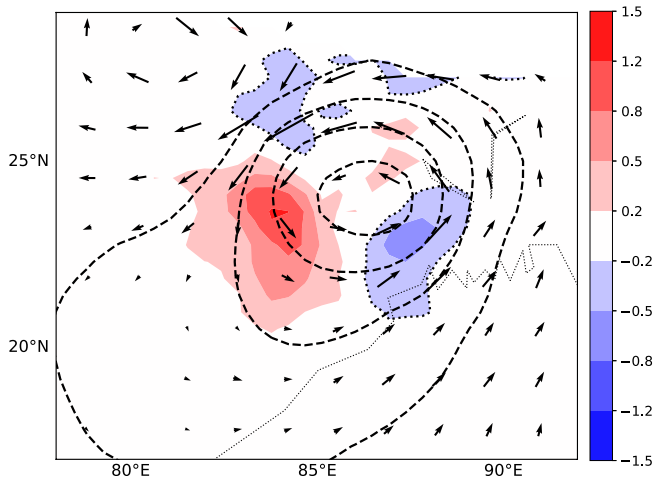
FIGURE 15 Experiment C. Perturbation vertical velocity ( w' , shading, cm/s, averaged from 1.2 to 5.3 km) and perturbation winds at 3.1 km ( v' , vectors) at 72 hr into the simulation. Negative values of w' are enclosed with a dotted line [Colour figure can be viewed at wileyonlinelibrary.com ]
