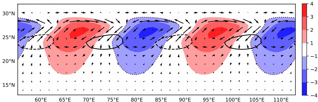
FIGURE 3 Perturbation pressure at 3.25 km ( p' , shading, hPa), perturbation winds at 3.25 km ( \mathbf{v}' , vectors), and perturbation vertical velocity averaged from 1.0 to 5.0 km ( w' , contours every 0.3 cm/s) for the 3,200 km wavelength normal mode from Experiment A. Negative values of p' are enclosed with a dotted line [Colour figure can be viewed at wileyonlinelibrary.com ]
