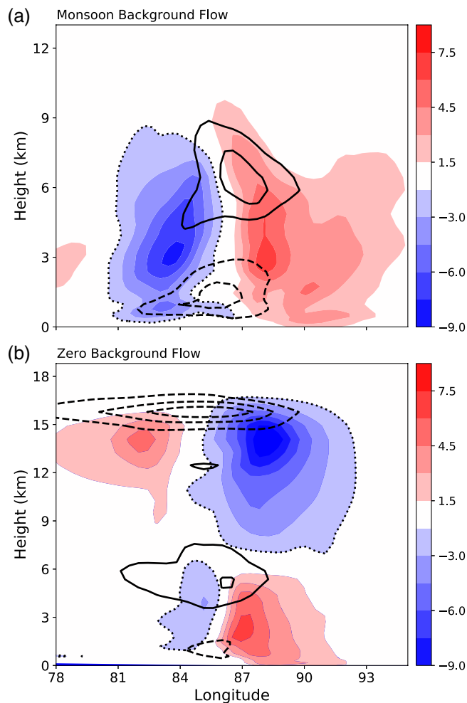
FIGURE 14 Experiment C. Longitude–height cross-section of the component of perturbation wind orthogonal to the cross-section (shading, m/s) and perturbation potential temperature ( \theta' , K, contours) at 3 days into the simulation for (a) monsoon basic state and (b) resting basic state. Negative values of v' are enclosed with a dotted line. This cross-section is rotated 30° clockwise from a line of constant latitude and the fields are averaged for 150 km on either side of the cross-section. Because of this rotation, longitude on the x -axis corresponds to 0.87 of its normal length. Note the change in the y -axis scale [Colour figure can be viewed at wileyonlinelibrary.com]
