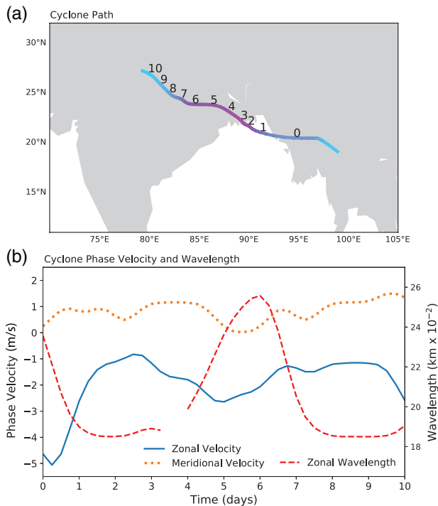
FIGURE 10 Experiment B. (a) track of the centre of the cyclonic phase of the wave disturbance with dates corresponding to Figure 7 and shaded by the magnitude of the pressure perturbation; lighter pinks correspond to lower pressure values and lighter blues to higher values. (b) zonal and meridional phase velocity and zonal wavelength as a function of time
